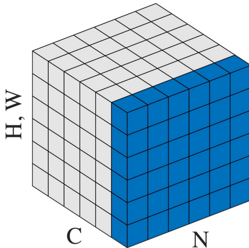
BatchNorm
