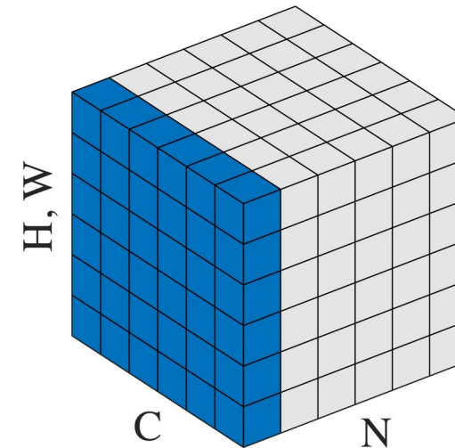
LayerNorm (shown here)
